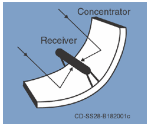
Figure 32. Diagram of a parabolic trough system, which concentrates solar heat onto an oil-filled pipe (OCS - Alternative Energy and Alternate Use Programmatic EIS Information Center).
