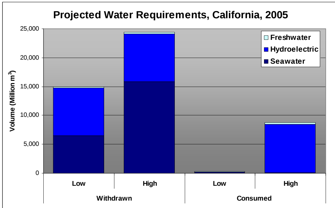
Figure 54. Projected water requirements for electricity generation in the State of California in 2005. These estimated withdrawals and consumption include freshwater (from surface and ground water sources), sea water, and freshwater in hydroelectric facilities.
