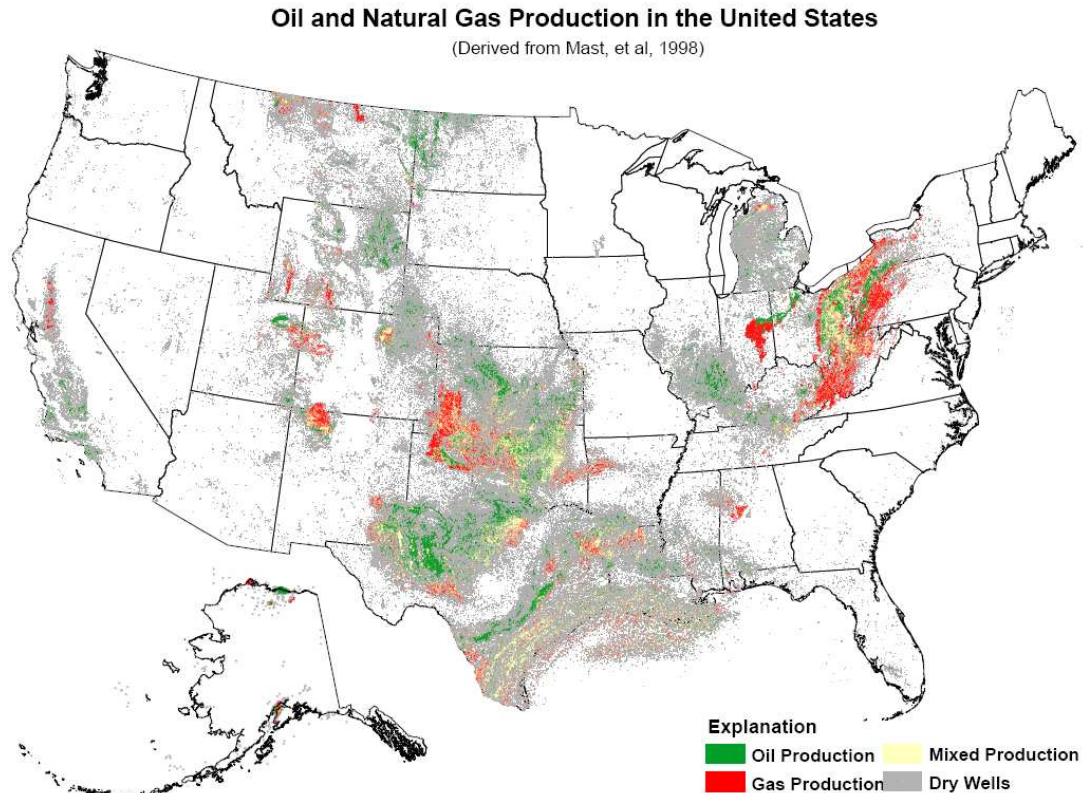
Figure 20. Map of oil and natural gas production in the United States (USGS, 2006b).
