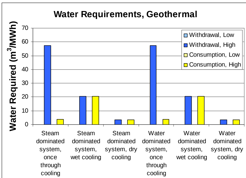
Figure 48. Water requirements from external sources for electricity generation in geothermal facilities. Low estimates of withdrawals and consumption are zero, which assumes that geothermal source fluids are captured and used for cooling or resource recharge.
